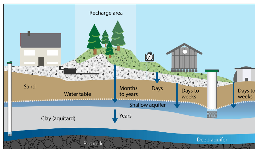
Figure 1. Aquifers and infiltration rates.
