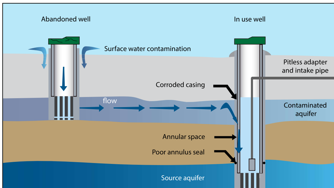
Figure 13. Surface water contamination from an abandoned well to a well in-use.
