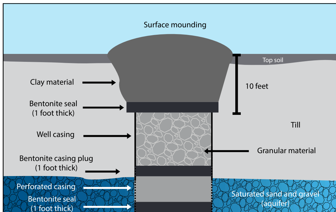
Figure 14. Completion of typical bored well decommissioning.
