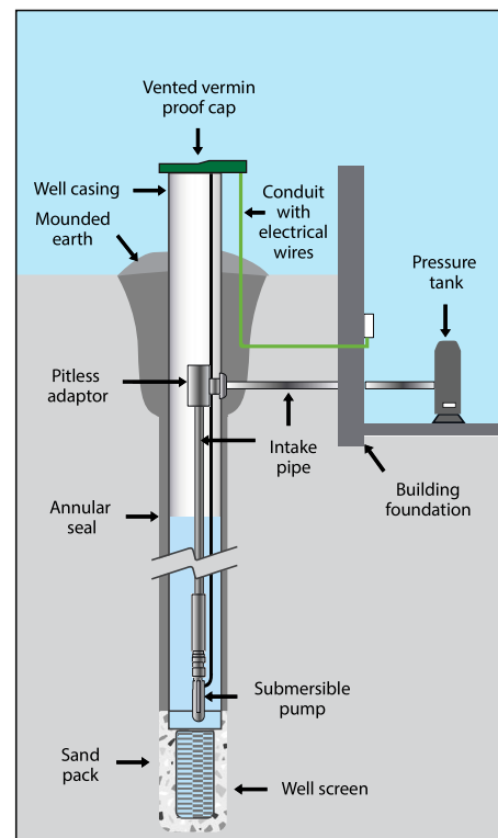
Figure 5. Small diameter drilled well.
