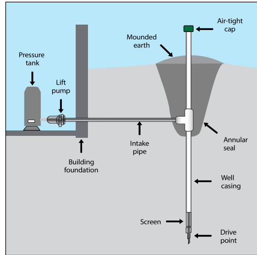
Figure 6. Driven point or sand point well.
